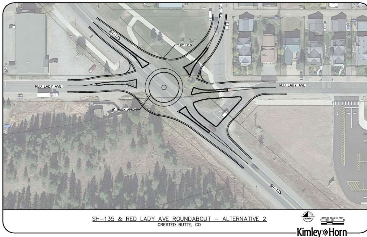
Figure 49 SH-135 & Red Lady Roundabout Intersection Concept Drawing
